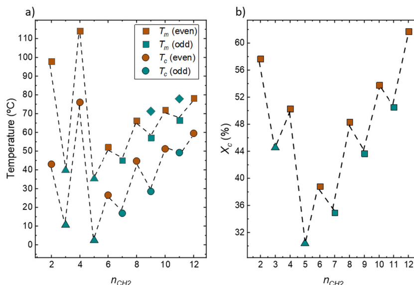
Fig. 4 (a) T_c and T_m as a function of the n_{CH_2} in the repeating unit of the PE_{nCH_2} s employed. The triangles represent the data obtained by micro-DSC, while the squares and circles represent the data obtained by DSC. The rhombus symbols indicate the second melting peak in PE9 and PE11. (b) X_c variation as a function of n_{CH_2} . A color code is used to distinguish even-numbered (brown) and odd-numbered (blue) samples.
