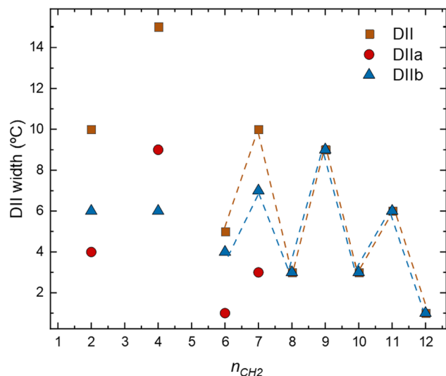
Fig. 12 Memory effect evaluation by taking the Domain II variation with chain length ( n_{CH_2} ).
