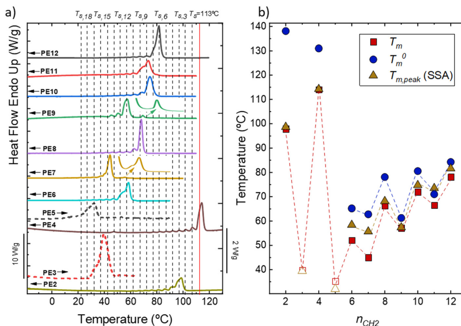
Fig. 13 (a) Final heating after the SSA protocol was applied to the indicated samples. We used the following conditions for the SSA protocol: T_{s,ideal} = 113 °C, a fractionation window of 5 °C, and scan rates of 20 °C min −1 . (b) T_m , T_m^0 and T_{m,peak} (SSA) as a function of n_{CH_2} .
