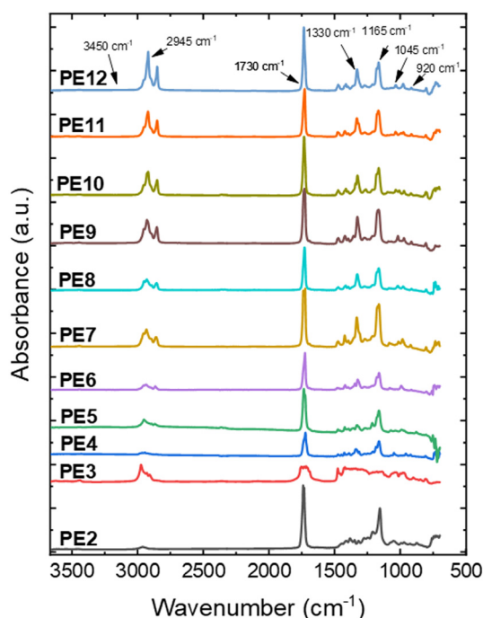
Fig. 6 Synchrotron FT-IR spectra of \text{PEnCH}_2\text{s} in the 3750 – 750 \text{ cm}^{-1} range at -40^\circ\text{C} after a cooling from the melt at 20^\circ\text{C min}^{-1} . PE3 and PE5 spectra was obtained at RT after an isothermal crystallization.
