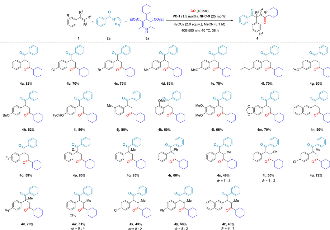
Scheme 2 Substrate scope of various alkenes, acyl imidazoles and Hantzsch esters to synthesize 1,4-diketones. Reaction conditions: 1 (0.2 mmol), 2 (0.4 mmol), 3 (0.5 mmol), MeCN (2.0 mL), K 2 CO 3 (0.4 mmol), 400–500 nm, isolated yield.
