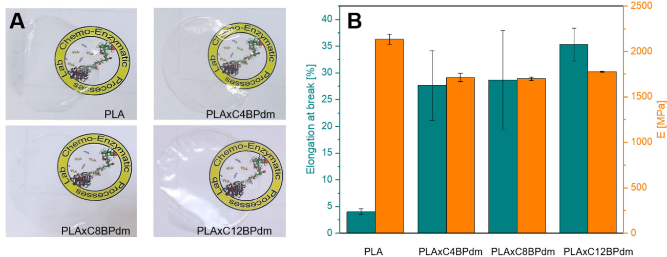
Fig. 5 Mechanical characterization of the obtained blended PLA films. (A) Photos of PLA and PLA BPdm-containing films: neat PLA, PLAxC4BPdm, PLAxC8BPdm, and PLAxC12BPdm. (B) Elongation at break ( \epsilon_{\text{break}} ) and Young's modulus ( E ) from the stress-strain test of PLA and PLA BPdm-containing films. Error bars represent the corresponding standard error.
