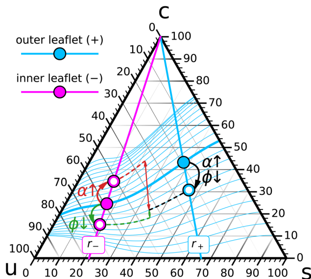
Fig. 5 Perturbation of a terynary asymmetric GUV initially set up such that its inner composition \{r_-, \phi_-\} (big magenta dot) and outer composition \{r_+, \phi_+\} (big cyan dot) chemically coexist at \mathcal{F} = 0 . The two independent perturbations which either decrease \phi or increase \alpha will have a similar effect on leaf _+ : a reduction of \phi_+ . But their effects on leaf _- are opposite: depleting cholesterol will reduce \phi_- while increasing \alpha will increase \phi_- . The extent to which this moves points that originally shared the same zero-torque foliation onto different foliation curves is very different.
