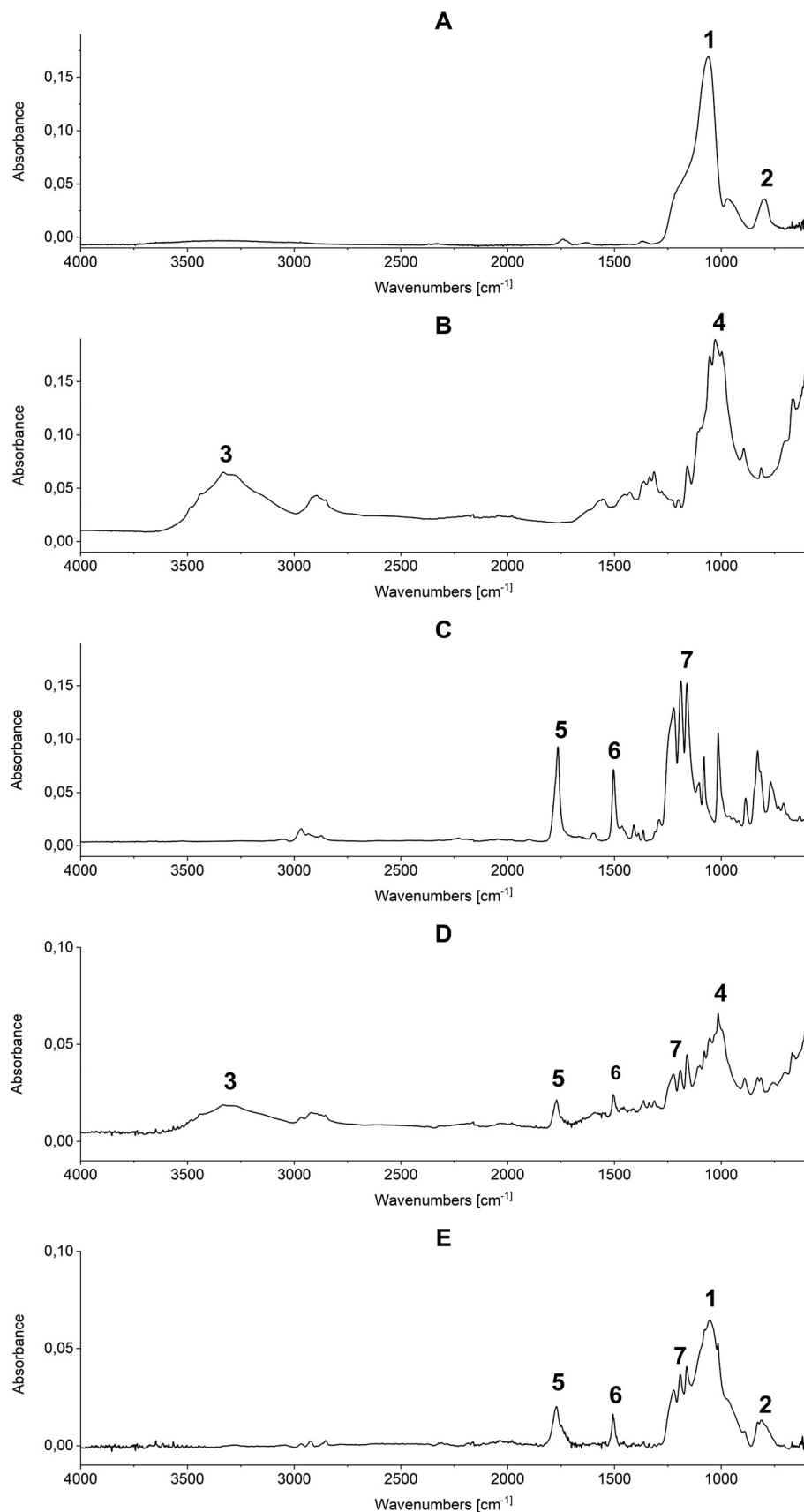
Fig. 3 FTIR spectra of prepared adsorbents. Optimization of cotton coverage with adsorption phase. The spectra are Aerosil (A), polycarbonate (C), bed with planned coverage of 30 \text{ mg cm}^{-2} PC/Aerosil (D) and with coverage of 36 \text{ mg cm}^{-2} PC/Aerosil (E). Description of marked bands, see section 3.2.
