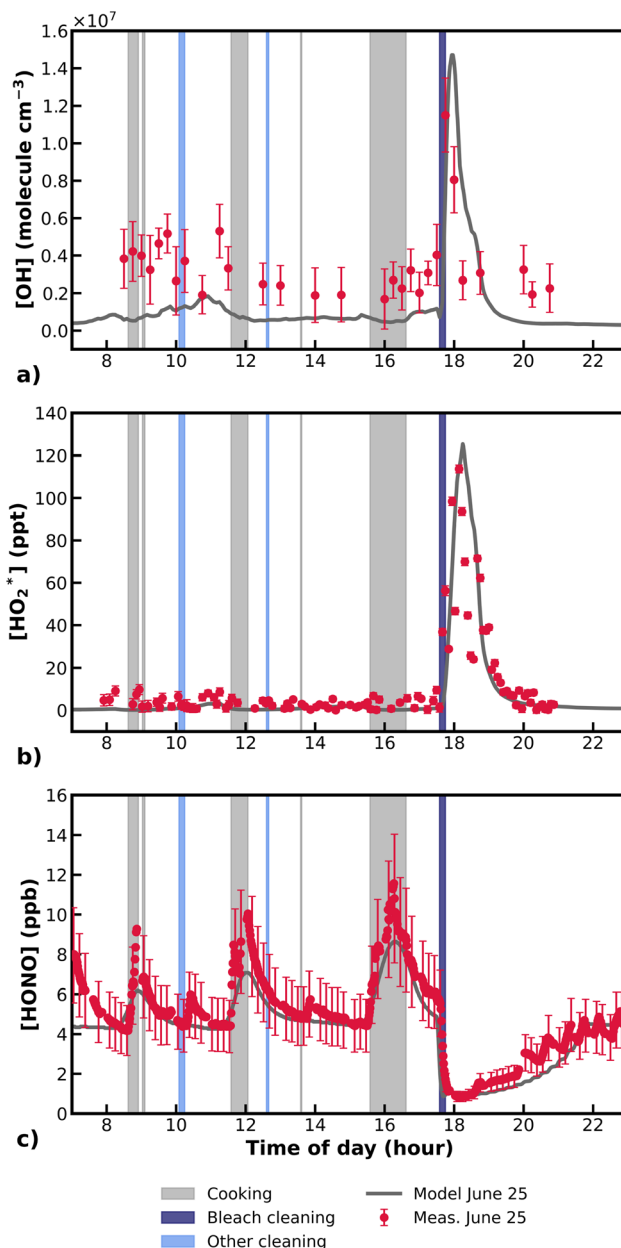
Fig. 2 Modelled (grey line) versus measured (red circles) concentrations of OH radicals (panel a, molecule per \text{cm}^3 ), HO 2 * radicals (panel b, ppt), and HONO (panel c, ppb) on June 25. Error bars represent the experimental uncertainties. The shaded areas indicate the timing of the activities carried out during the day: cooking (grey), Cl-cleaning (dark blue), and other cleaning (light blue) activities.
