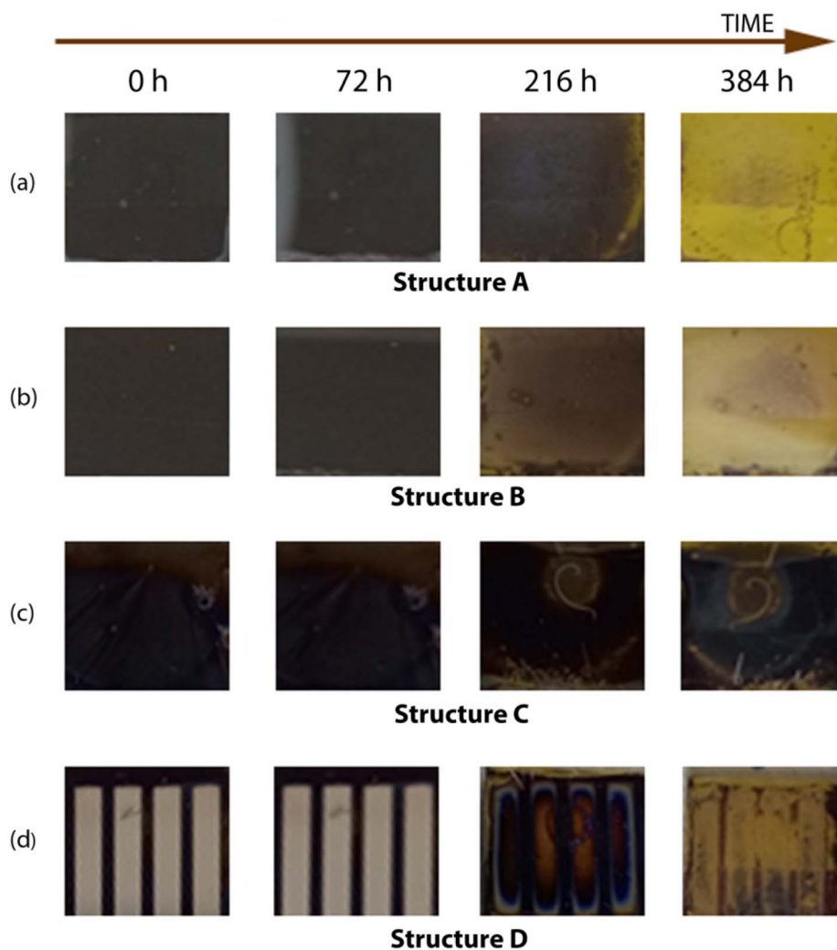
Fig. 2 Photographs showing the stability of (a) structure A: FTO/MAPbI 3 , (b) structure B: FTO/NiO x /MAPbI 3 , (c) structure C: FTO/NiO x /MAPbI 3 /PCBM, and (d) structure D: FTO/NiO x /MAPbI 3 /PCBM/Ag as a function of storage time in air with a relative humidity of \sim 60 \pm 8\% . The FTO substrate size was 1.8 \times 1.5 cm 2 .
