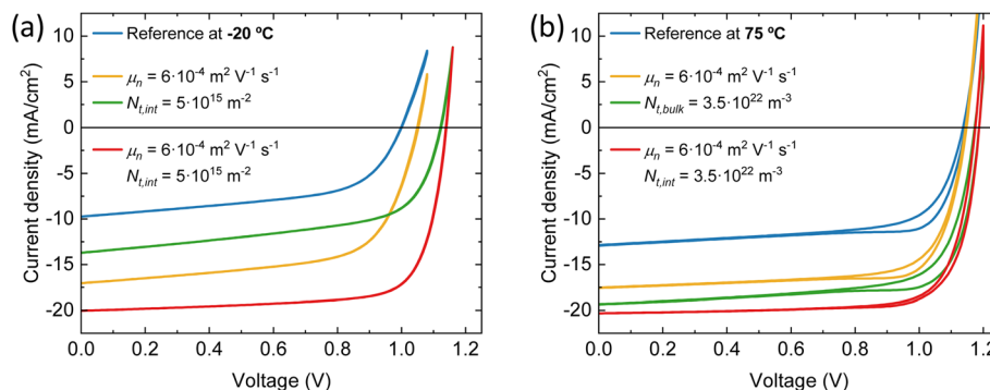
Fig. 6 Simulated J-V curves at 1 sun eq. at (a) -20\text{ }^{\circ}\text{C} substrate temperature for different electron mobility and trap density at both interfaces (b) 75\text{ }^{\circ}\text{C} substrate temperature for different electron mobility and bulk trap density.
