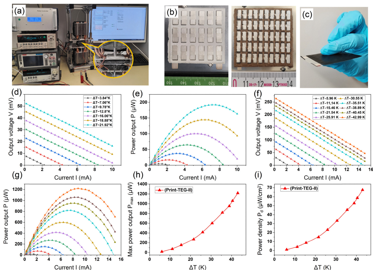
Fig. 5 (a) Experimental setup for V - I characterization using the SMU unit. (b) Top view of the print-TEG I & print-TEG II devices for visual representation. (c) Lateral view of the print-TEG II insulated with carbon tape. (d) V - I characteristics of print-TEG I at \Delta T s. (e) P - I characteristics of print-TEG I at \Delta T s. (f) V - I characteristics of print-TEG II at \Delta T s. (g) P - I characteristics of print-TEG II at \Delta T s. (h) Max power output P_{\text{max}} of print-TEG II at \Delta T s. (i) Power density P_d of print-TEG II at \Delta T s.
