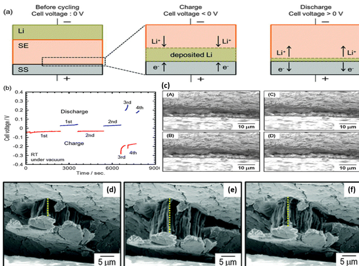
Fig. 30 In situ SEM measurements at different CD. (a) Schematic diagrams illustrating the Li/SE/SS cells before the cycle and a detailed view of the interface between the solid electrolyte and stainless steel during charging and discharging. (b) Li deposition and dissolution curves for Li/SE/SS are presented at a CD of 0.01 mA cm -2 during the first and second cycles and at 0.05 mA cm -2 during the third and fourth cycles. (c) SEM images of the interface show conditions (A) after the first charge, (B) after the first discharge, (C) after the second charge, and (D) after the second discharge. SEM images of the SE/stainless steel interface at a similar location within a similar configuration are shown (d) instantly following a short circuit, (e) during Li deposition via 5 mA cm -2 for 10 min after the short circuit, and (f) during Li dissolution via 20 mA cm -2 for 20 min shortly after (e). 200
