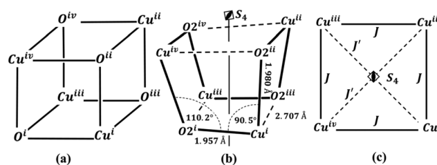
Fig. 6 (a) Ideal cubane \text{Cu}_4\text{O}_4 core ( T_d symmetry). (b) Cubane-like \text{Cu}_4\text{O}_4 core in the tetranuclear \text{Cu}_4\text{L}_4 complex (crystallographic site symmetry S_4 , a subgroup of T_d ) showing super-exchange relevant Cu–O bond paths (in full lines), distances (Å) and Cu–O–Cu bond angles ( ^\circ ). Some weaker Cu...O paths are indicated by thin lines. Symmetry operations as in Fig. 3. (c) Exchange coupling scheme used in the spin Hamiltonian of eqn (2).
