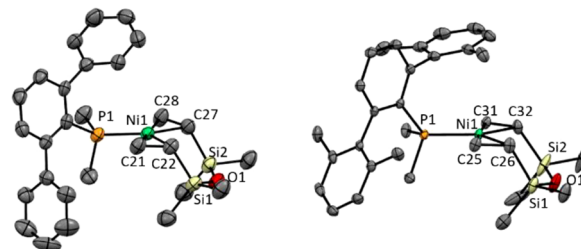
Scheme 3 (A) Synthesis of [\text{Ni}(\text{PR}_2\text{Ar}')(\text{DVDS})] complexes 5–9 . (B) Molecular structures of 5 (left) and 6 (right). Hydrogen atoms are omitted for the sake of clarity. Thermal ellipsoids are shown at a 50% probability. Selected bond lengths [Å] and angles [°] for 5 : Ni1–P1 2.162(1), Ni1–C21 1.986(4), Ni1–C22 2.000(4), Ni1–C27 2.019(3), Ni1–C28 1.995(3), C21–C22 1.398(6), C27–C28 1.293(5), P1–Ni1–C21 92.1(1), P1–Ni1–C22 132.4(1), P1–Ni1–C27 133.1(1), P1–Ni1–C28 93.2(1); for 6 : Ni1–P1 2.1669(8), Ni1–C25 1.998(2), Ni1–C26 2.008(2), Ni1–C31 2.017(2), Ni1–C32 1.990(2), C25–C26 1.411(4), C31–C32 1.406(3), P1–Ni1–C25 91.67(8), P1–Ni1–C26 132.58(8), P1–Ni1–C31 133.74(7), P1–Ni1–C32 92.70(7).
