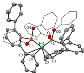
Scheme 2 (A) Synthesis of \text{NiP}_2 complexes 3 and 4 . (B) Improved synthetic route for [\text{Ni}(\text{PMe}_2\text{Ar}^{\text{DtbP}2})_2] , 2 . (C) Molecular structure of 4 . Hydrogen atoms are omitted for the sake of clarity. Thermal ellipsoids are shown at a 50% probability. Selected bond lengths [Å] and angles [°]: Ni–P1 2.1253(5), Ni–P2 2.1074(5), Ni–C1 2.086(2), Ni–C2 2.211(2), Ni–C3 2.614(2), Ni–C4 2.4261(2), P1–Ni–P2 115.37(2).
