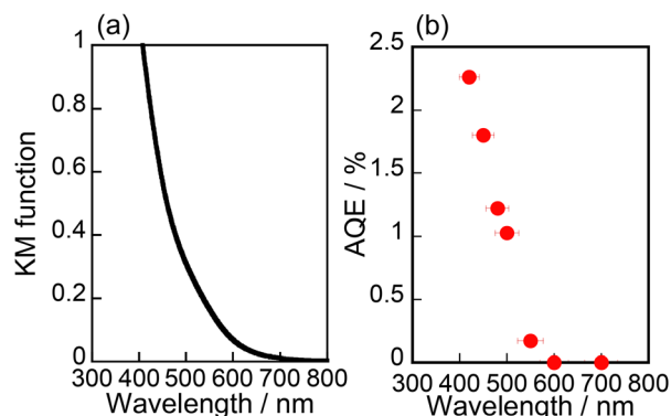
Fig. 6 (a) UV-vis diffuse reflection spectra of \text{RhO}_x/\text{TiO}_2(500-400) , and (b) action spectrum of \text{RhO}_x/\text{TiO}_2(500-400)\text{-Pt} in formation of \text{H}_2 from 2-propanol.
