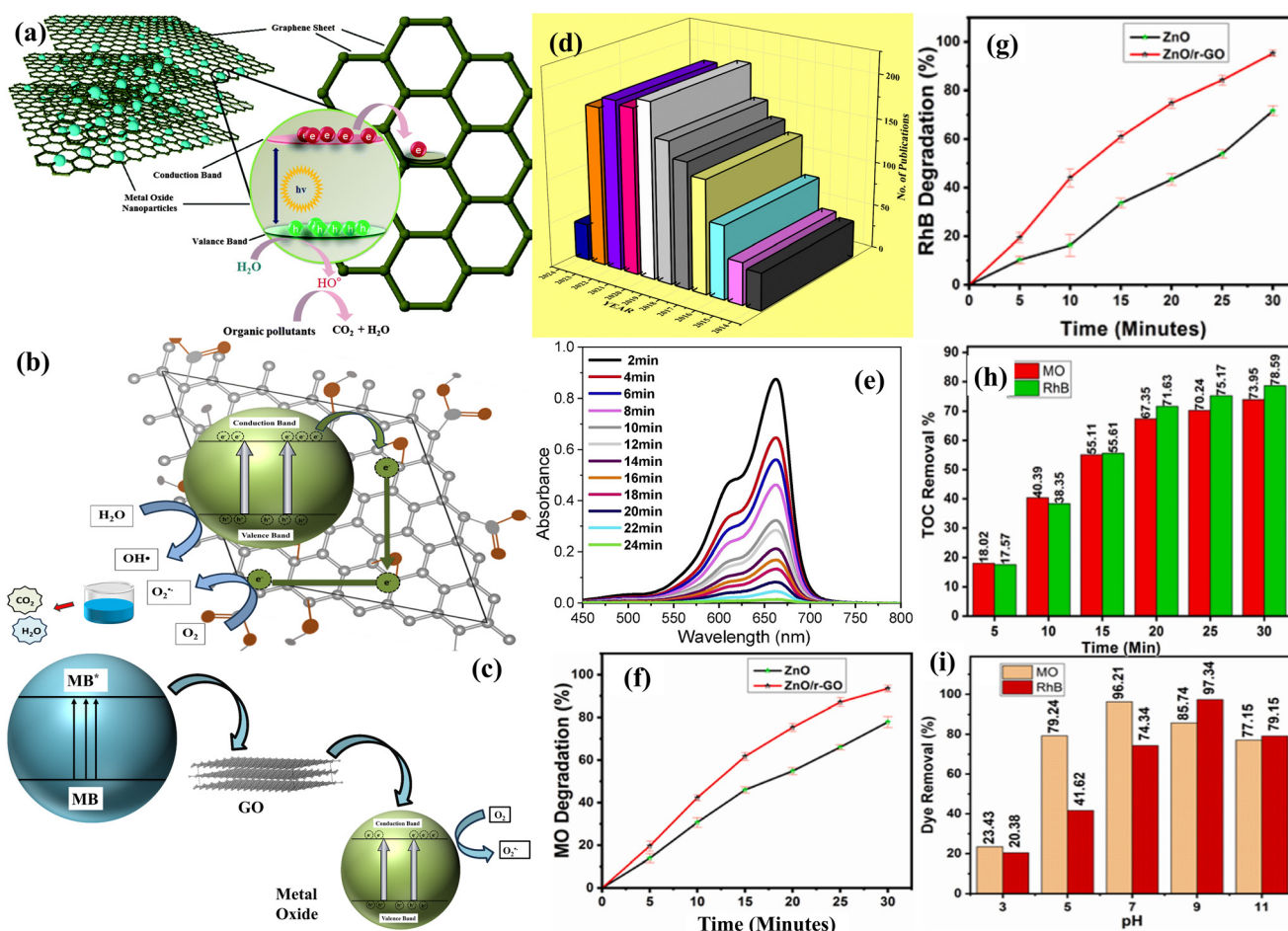
Fig. 6 (a) Electron transfer from the CB of a metal oxide to graphene via a percolation mechanism. Reproduced with permission from ref. 163 Copyright (2024), Elsevier. (b) Chemical mechanism involving the photodegradation of dyes by GO metal oxide photocatalysts, highlighting the function of GO as a charge carrier to boost the photocatalytic efficacy of GO-metal oxide nanocomposites. (c) Schematic of the efficient charge transfer facilitated by GO from dye molecules to metal oxide photocatalysts. (d) Statistical data for the number of publications on metal oxide-based GO nanocomposite for various applications. (e) Photocatalytic degradation of MB using GO/ZnO nanocomposite. Reproduced with permission from ref. 163 Copyright (2024), Elsevier. (f) Degradation of MO and (g) RhB dyes by ZnO and rGO/ZnO composite. (h) Evaluation of TOC removal during the degradation of MO and RhB by rGO/ZnO nanocomposites. (i) Investigation of the impact of initial pH on the photocatalytic degradation of MO and RhB. Reproduced with permission from ref. 164 Copyright (2022), Elsevier.
