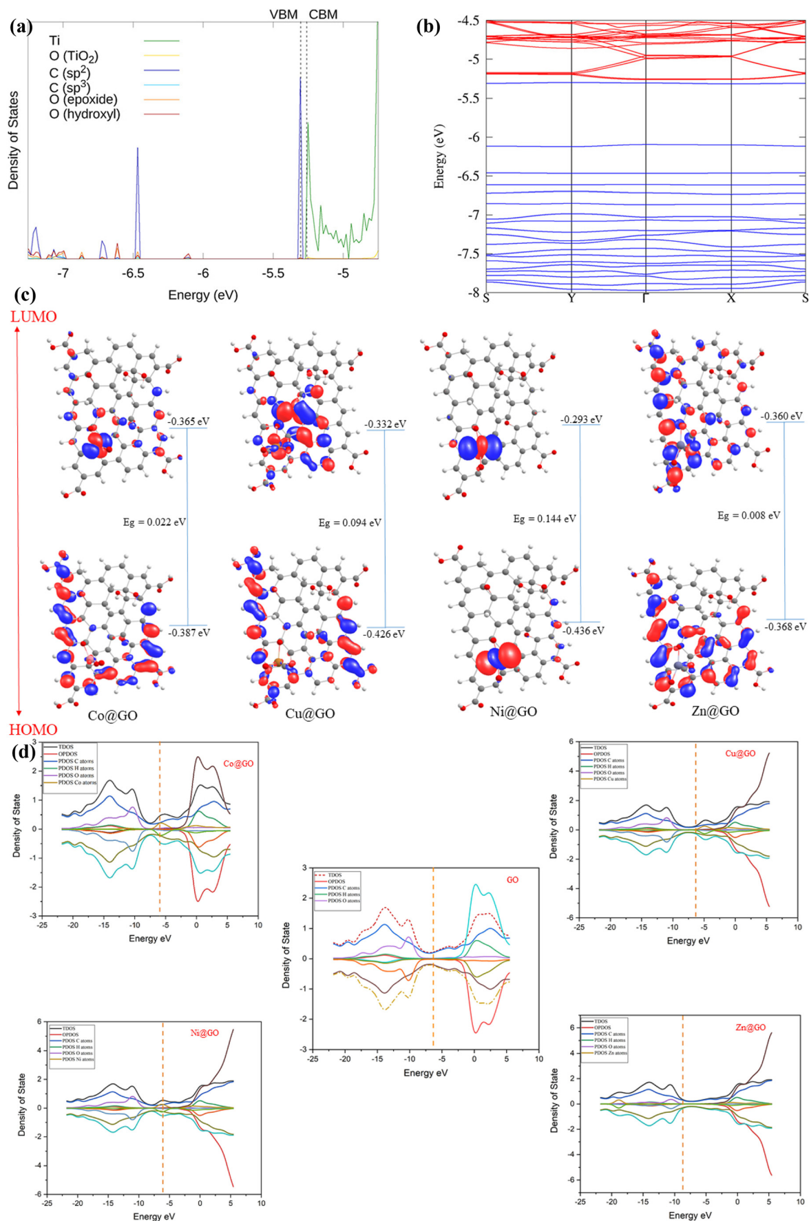
Fig. 20 (a) DOS spectrum of GO/rutile (110) TiO 2 . (b) Band structure of GO/rutile (110) TiO 2 . 431 (c) Iso-surface HOMO and LUMO and (d) visualization of the density of states for Co@GO, Cu@GO, Ni@GO and Zn@GO. 432
