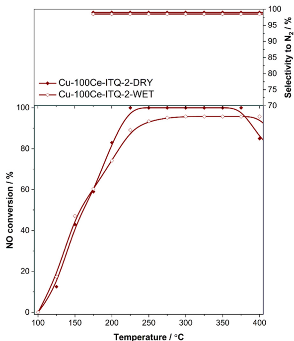
Fig. 13 Temperature dependence of catalytic NH 3 -SCR activity of the Cu-Ce-ITQ-2 catalyst under dry and humid (5 vol% H 2 O) conditions (GHSV of 17 000 h -1 ).
