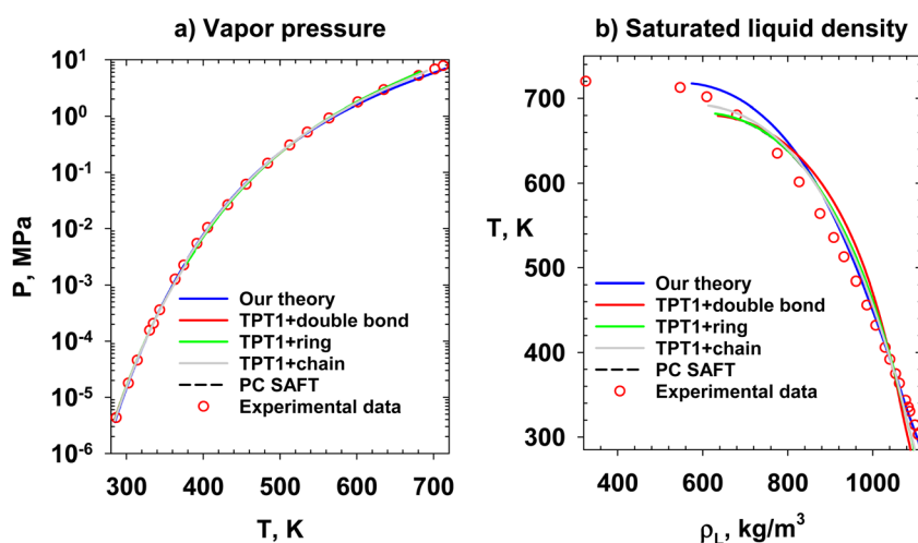
Fig. 19 (a) Saturation pressure and (b) saturated liquid density of MEG. Blue, red, green, gray, and dashed black lines represent association theories based on our theory, TPT1 + double bond, TPT1 + ring, TPT1 + chain, and PC SAFT. Point represents experimental data. 31
