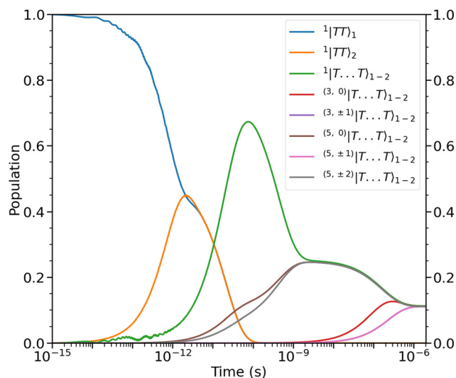
Fig. 4 Populations as a function of time of the intrachain states, |1^1TT\rangle_1 and |1^1TT\rangle_2 , and interchain states, |^{(2S+1, M_S)}T \cdots T\rangle_{1-2} . The dynamics can be divided into four time regimes, which are described in the main text. States of same spin and magnitude of M_S are populated simultaneously. Note that the rate of population of the triplet and quintet states with M_S = \pm 1 are similar enough that the two lines corresponding to those populations (purple and pink) overlap. At ca. 2 \mu s the nine lowest energy levels (illustrated in Fig. 3) are equally populated.
