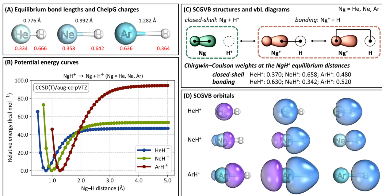
Fig. 1 (A) Optimised geometries at the \text{CCSD}(\text{T})/\text{aug-cc-pVTZ} level of theory and ChelpG atomic charges of noble gas hydrides \text{NgH}^+ ( \text{Ng} = \text{He} - \text{Ar} ). The computed equilibrium bond lengths are given in black, while the ChelpG charges are given in red. (B) Potential energy curves of the \text{NgH}^+ systems at the \text{CCSD}(\text{T})/\text{aug-cc-pVTZ} level. Energies are presented relative to the minimum point in each curve. (C) SCGVB structures and valence-bond-Lewis (vbl) diagrams representing the three resonance structures considered in our SCGVB wave functions, blocked into closed-shell ( \text{Ng} + \text{H}^+ ) and bonding ( \text{Ng}^+ + \text{H} ) contributions. (D) Optimised SCGVB orbitals at the \text{SCGVB}(2,3)/\text{aug-cc-pVTZ}/\text{CCSD}(\text{T})/\text{aug-cc-pVTZ} orbitals.
