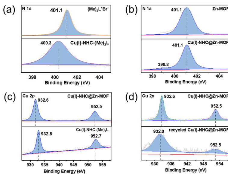
Fig. 3 (a) XPS spectra of N 1s in \text{Cu}(\text{I})\text{-NHC}-(\text{Me})_2\text{L} and (\text{Me})_2\text{L}^+\text{Br}^- ; (b) N 1s in Zn-MOF and \text{Cu}(\text{I})\text{-NHC@Zn-MOF} ; (c) Cu 2p in \text{Cu}(\text{I})\text{-NHC@Zn-MOF} and \text{Cu}(\text{I})\text{-NHC}-(\text{Me})_2\text{L} ; (d) Cu 2p in \text{Cu}(\text{I})\text{-NHC@Zn-MOF} and recycled \text{Cu}(\text{I})\text{-NHC@Zn-MOF} .
