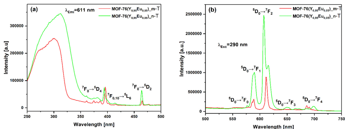
Fig. 16 (a) Excitation ( \lambda_{\text{Emi}} = 611 \text{ nm} ) and (b) emission spectra ( \lambda_{\text{Exc}} = 290 \text{ nm} ) of MOF-76( \text{Y}_{0.95}\text{Eu}_{0.05} ) n-T and MOF-76( \text{Y}_{0.95}\text{Eu}_{0.05} ) m-T materials.
