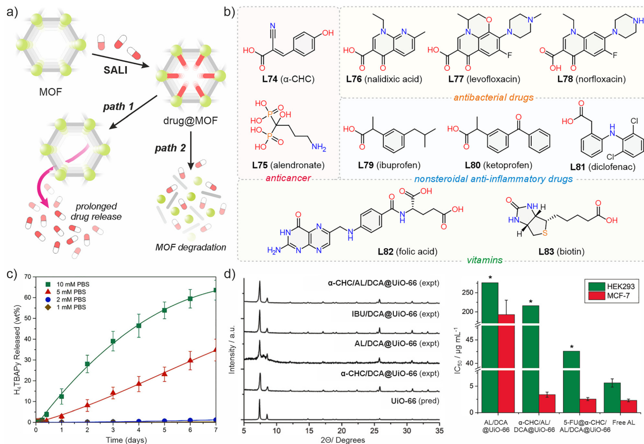
Fig. 9 (a) Scheme of the preparation of SALI-based drug delivery system (drug@MOF) and two possible pathways of drug release: path 1 based on slow discooordination of introduced molecules (reverse-SALI) and path 2 where MOF degradation leads to more rapid drug release. 169 (b) Examples of bioactive molecules introduced into MOF via SALI technique; \alpha -CHC = \alpha -cyano-4-hydroxycinnamic acid. (c) Stability in different concentrations of PBS of representative Zr-MOF (NU-1000) studied as drug delivery system. 169 Reprinted from ref. 169 with permission. Copyright 2018 Elsevier. (d) Powder X-ray diffraction (PXRD) patterns of drug-loaded UiO-66 (left) and comparison of IC_{50} values of drug-loaded UiO-66 compared with free alendronate (AL) against HEK293 and MCF-7 cell lines. 45 Figure adapted from ref. 45 with permission. Copyright 2020 John Wiley and Sons.
