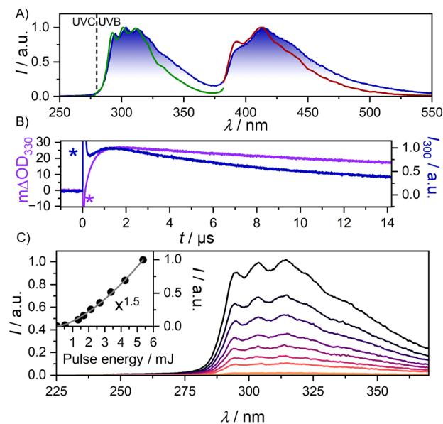
Fig. 4 Mechanistic investigations of 25 \mu\text{M} Ir and 2 mM TIPS-Bz in Ar-saturated benzene. (A) Time-gated emission spectrum after 355 nm laser excitation (blue, 4–204 \mu\text{s} ) and after 280 nm excitation (green and red, normalized to the maximum in the UV and visible region). (B) Kinetic traces of the 1 TIPS-Bz * emission and transient absorption of 3 TIPS-Bz . (C) Excitation-intensity dependent delayed emission spectra. Inset: Emission maximum plotted against laser pulse intensity with a pulse duration of \sim 5 ns. See text for details.
