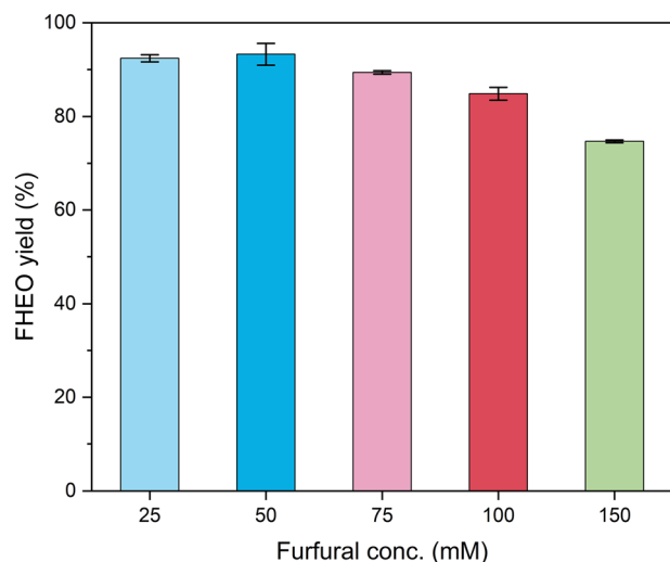
Fig. 1 Biocatalytic FHEO synthesis at different substrate loadings. Reaction conditions: 25–150 mM furfural, 1.5 equiv. formaldehyde, 25 g L -1 E. coli - SulPDC cells (wet weight), 0.15 mM ThDP, 2.5 mM Mg 2+ , 1 mL phosphate buffer (50 mM, pH 6), 35 °C, 150 rpm, 10 h. Notably, the reaction time is 24 h at 100–150 mM substrate loadings.
