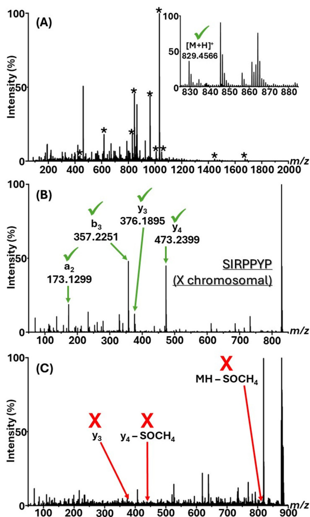
Fig. 3 LAP-MALDI MS and MS/MS spectra for the tooth of skeleton 106 (female; cf. Table 1). (A) LAP-MALDI MS profile with inset displaying the m/z region for the singly charged SM_{ox} IRPPY (Y chromosome) and SIRPPYP (X chromosome) peptides. Ion signals obtained from peptides extracted from the tooth are labeled by asterisks. (B) LAP-MALDI MS/MS spectrum of the precursor ions at m/z 829.5 (singly protonated SIRPPYP). (C) LAP-MALDI MS/MS spectrum of the precursor ions at m/z 879.4.
