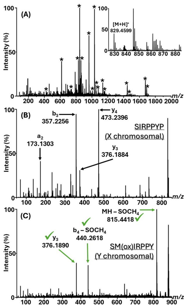
Fig. 2 LAP-MALDI MS and MS/MS spectra for the tooth of skeleton 136 (male; cf. Table 1). (A) LAP-MALDI MS profile with inset displaying the m/z region for the singly charged SM_{ox} IRPPY (Y chromosome) and SIRPPYP (X chromosome) peptides. Ion signals obtained from peptides extracted from the tooth are labeled by asterisks. (B) LAP-MALDI MS/MS spectrum of the precursor ions at m/z 829.5 (singly protonated SIRPPYP). (C) LAP-MALDI MS/MS spectrum of the precursor ions at m/z 879.4 (singly protonated SM_{ox} IRPPY).
