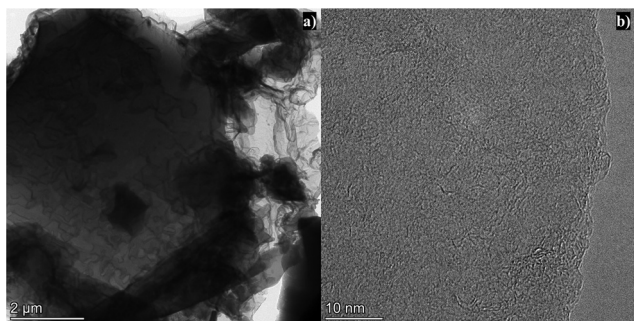
Fig. 2 (a) Transmission electron micrograph and (b) high-resolution transmission electron micrograph of L N-K.
