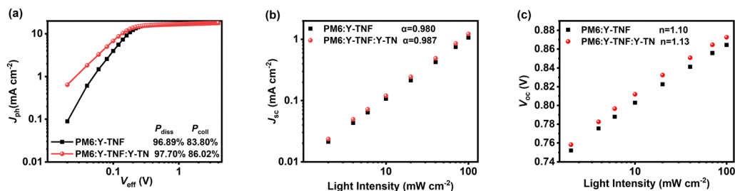
Fig. 4 (a) J_{\text{ph}}-V_{\text{eff}} curves, (b) J_{\text{sc}}-P_{\text{light}} and (c) V_{\text{oc}}-P_{\text{light}} of the binary device based on PM6:Y-TNF and the ternary device based on PM6:Y-TNF:Y-TN (1:1:0.1, w/w/w).
