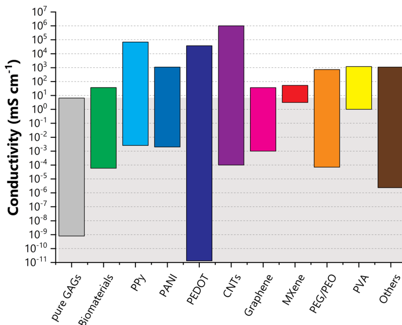
Fig. 10 Conductivity values found in the literature for pure GAG materials (in grey), as well as GAG associations with biomaterials (green), conductive polymers (poly(pyrrrole) (PPy) in light blue; poly(aniline) (PANI) in blue; poly(3,4-ethylenedioxythiophene) (PEDOT) in dark blue); carbon nanomaterials (carbon nanotubes (CNTs) in purple; graphene and derivatives in magenta; MXene in red), poly(ethylene glycol) (PEG)/poly(ethylene oxide) (PEO) in orange; poly(vinyl alcohol) (PVA) in yellow; and other precursors in brown.
