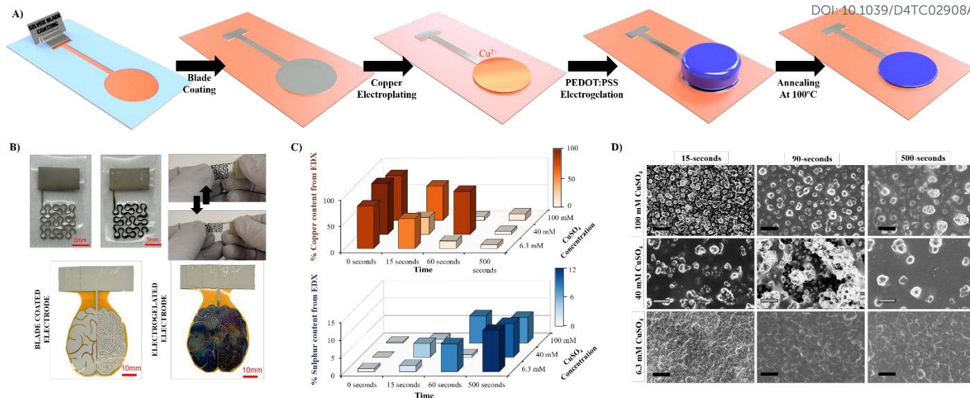
Figure 1. A) Electrode manufacturing process. Silver nanoparticle paste is blade coated on the substrate (e.g., Kapton) using a silicon-based tape mask, copper is electroplated on the silver electrode, the electrode is immersed in 10 v/v% PEDOT:PSS dilution and the copper is oxidized at 0.5 V forming a gel. Finally, the gel is collapsed via annealing for 5 min at 100°C, B) Examples of electrodes bladed coated (grey) with silver ink and after electrogelation (blue) on polyurethane (top) and Kapton (bottom), C) Bar graph of EDX elemental analysis of electrodes electrogelated at different times and under different copper salt conditions, orange for the percentage of copper and blue for the percentage of sulphur and D) SEM morphologies for different electrogelation times and copper electroplating concentrations.
