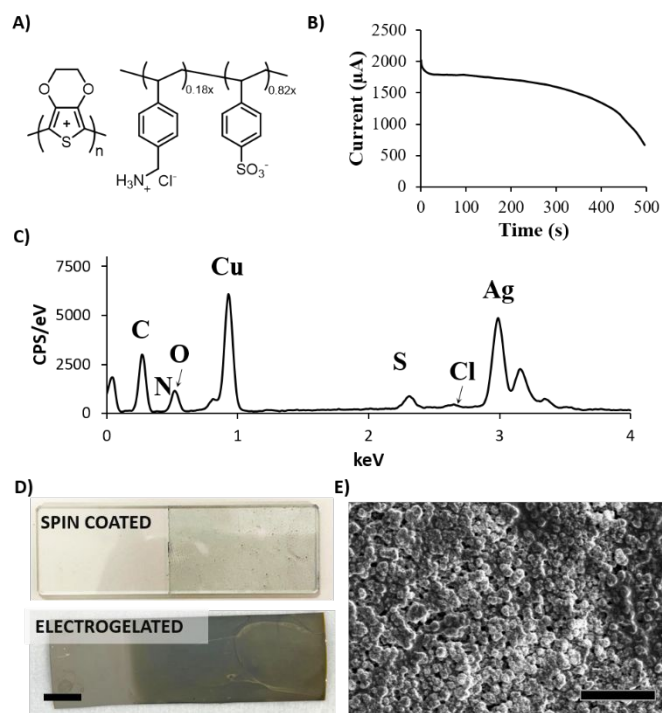
Figure 5. A) Chemical structure of PEDOT:PSS-co-PSMA, B) Chronoamperometry of the electrogelation during 500-sec using 6.3 mM electroplated electrodes, C) SEM-EDX of the sample, indicating the presence of the elements, D) Comparative photo of PEDOT:PSS-co-PSMA spin coated (top) and 500-sec electrogelated (scale bar: 1 cm) and E) SEM of Ag/Cu/PEDOT:PSS-co-PSMA electrodes (scale bar: 10 \mu\text{m} ).
