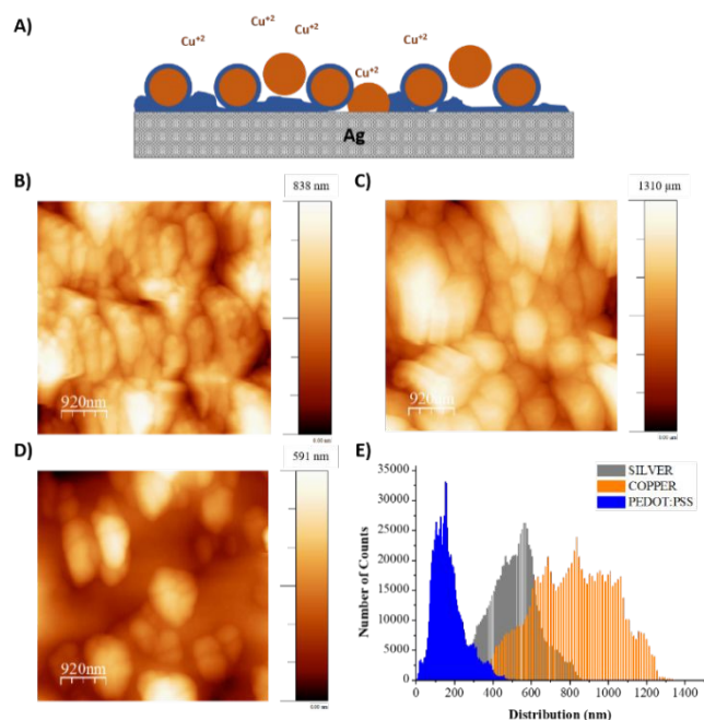
Figure 2. A) Diagram describing the behaviour of PEDOT:PSS electrogelation for low copper concentrations (6.3 and 40 mM of \text{CuSO}_4 ), AFM of B) Ag electrode, C) Ag/Cu electrode using 6.3 mM \text{CuSO}_4 and D) Ag/Cu/15-sec PEDOT:PSS electrode and E) Root mean square (RMS) roughness of the three electrodes.
