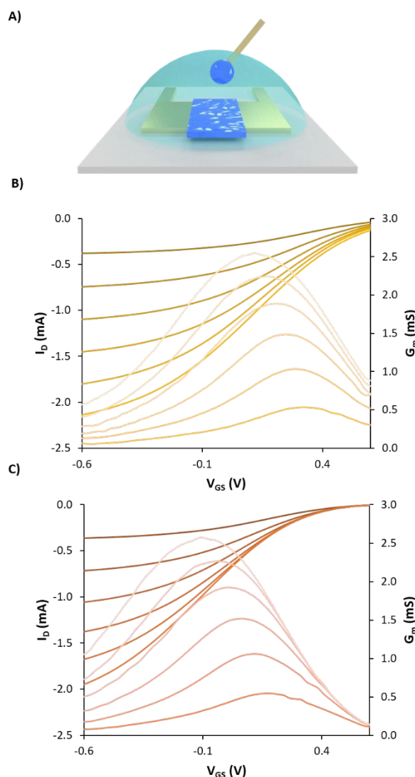
Figure 6. A) Schematic representation of an OECT; PEDOT:PSS is deposited on the channel between the drain and source while the electrogelated Ag/Cu/PEDOT:PSS-co-PSMA is used as gate electrode. Transfer-characteristics and transconductance curves at varying drain voltages from 0 to -0.6 V of OECTs with a channel of L = 600\mu\text{m} , W = 70 \mu\text{m} , of B) bare gold gate and C) Ag/Cu/PEDOT:PSS-co-PSMA (C) gate. For all cases, R = 2\text{mm} and the V_D is set from -0.1 to -0.6 V with an interval of 0.1 V
