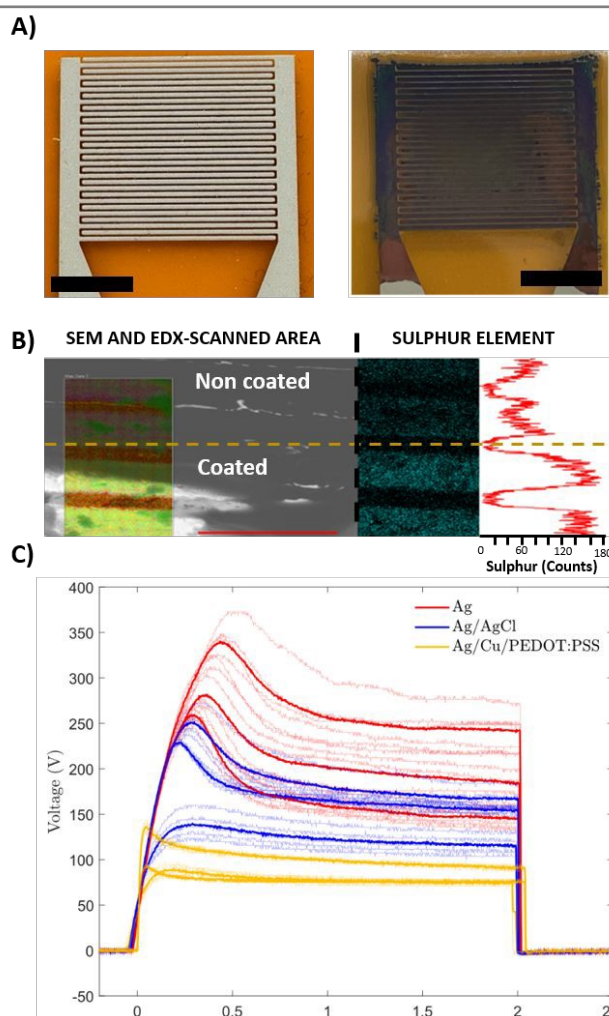
Figure 3. A) Optical image of pristine and PEDOT:PSS coated FIDE (scale bar: 4 mm), B) SEM-EDX spectroscopy of FIDE fingers. The top two fingers were not coated with PEDOT:PSS, observing a lower sulphur count, compared to the bottom fingers, coated with PEDOT:PSS where a greater count number is appreciated and C) Voltage applied to inject 1.3 mA of current using 2 ms pulses. Three Ag/AgCl devices (blue), three silver (red) and three Ag/Cu/PEDOT:PSS (gold) electrodes are compared. Thick tracks correspond to the averaging for each device, while thin traces correspond to each individual stimulation.
