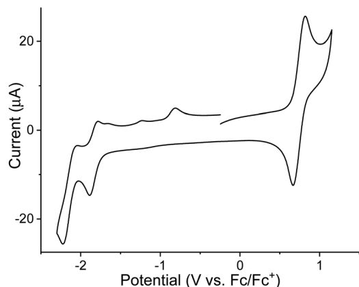
Fig. 2 Cyclic voltammetry for compound 1 in 1,2-dichlorobenzene solution (ca. 10^{-5} M), in the presence of 10^{-1} M ( n -Bu 4 N)(PF 6 ) as a supporting electrolyte measured at a scan rate of 100 \text{ mV s}^{-1} .
