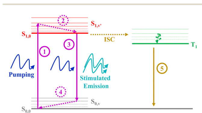
Fig. 5 Scheme depicting the 4-level scheme for successful ASE and the effect of triplet level addition.
