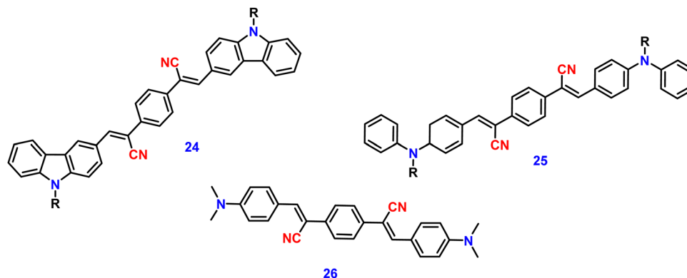
Fig. 18 Structure of compounds 24–26 .
