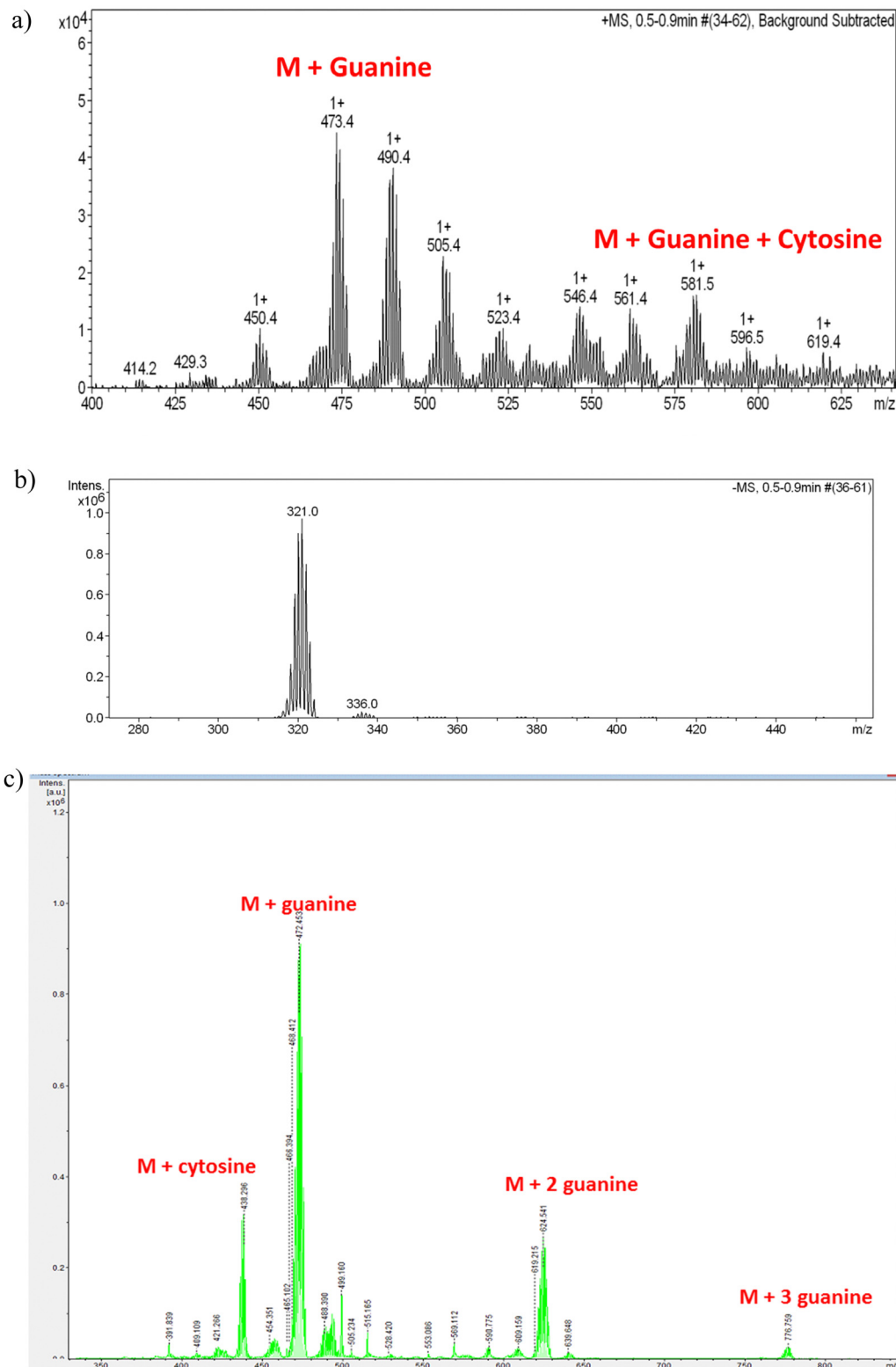
Fig. 8 (a) Magnification of the ESI-MS spectrum of the CT-dsDNA/Na[o-FESAN] nanohybrid at the positive mode in the range 400–650 m/z with isotopic (+1) distribution; Fig. S8 at the ESI \dagger displays the full spectrum in the range 0–1200 m/z . (b) ESI-MS spectrum of the CT-dsDNA/Na[o-FESAN] nanohybrid at the negative mode with isotopic (–1) distribution in the range 270–470 m/z ; only molecular peak of the [o-FESAN] ^- at 321.0. (c) MALDI-TOF-MS of the nanohybrid CT-dsDNA/Na[o-FESAN] using DHB (2,5-dihydroxybenzoic acid) matrix at the anode with 30% attenuation.
