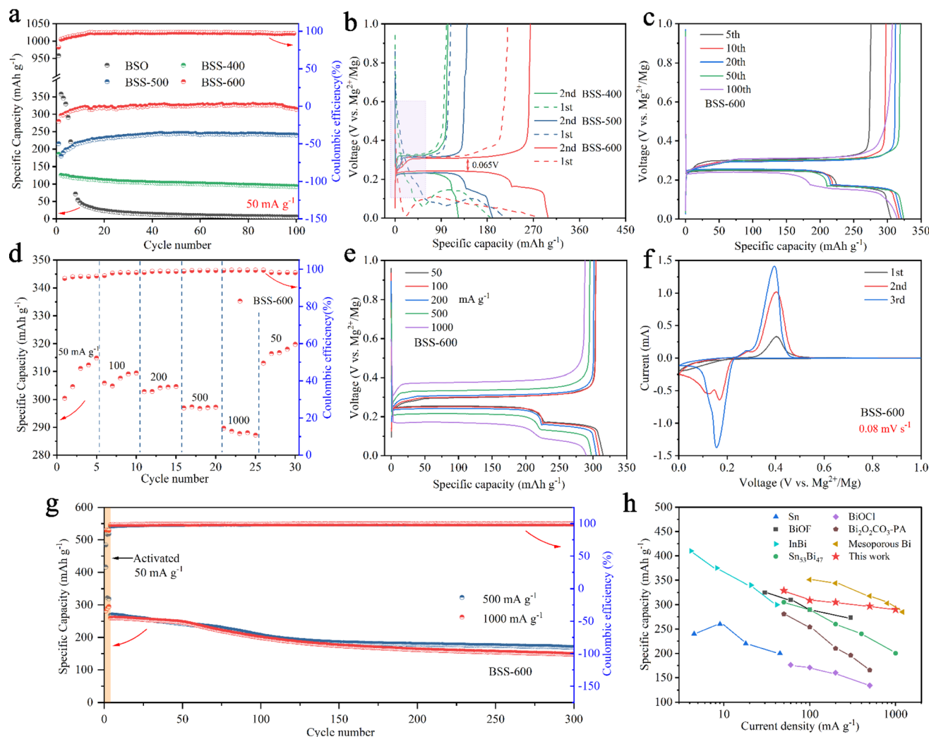
Fig. 4 (a) Cycling performance of the as-prepared samples at 50 mA g -1 . (b) The first two discharge/charge curves of BSS-400, BSS-500 and BSS-600 corresponding to (a). (c) Discharge/charge profiles of the BSS-600 electrode after different cycles. (d) Rate performance and (e) corresponding discharge/charge curves of the BSS-600 electrode at different current densities. (f) CV curves of the BSS-600 electrode and (g) cycling performance of the BSS-600 electrode at 500 mA g -1 and 1 A g -1 . (h) The comparison of rate performance in this work with the reported data in the literature.
