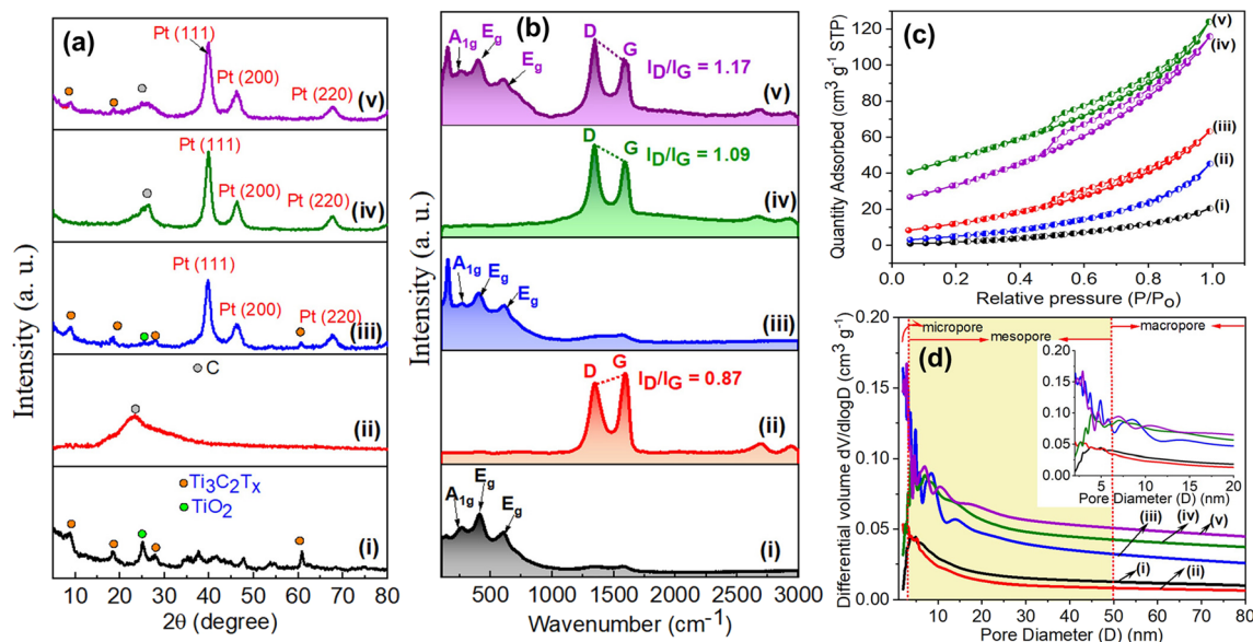
Fig. 2 (a) X-ray diffraction pattern, (b) Raman spectra, (c) \text{N}_2 adsorption–desorption isotherms, and (d) pore size distribution curve of (i) \text{Ti}_3\text{C}_2\text{T}_x , (ii) rGO, (iii) \text{Pt@Ti}_3\text{C}_2\text{T}_x , (iv) \text{Pt@rGO} and (v) \text{Pt@Ti}_3\text{C}_2\text{T}_x\text{-rGO} .
