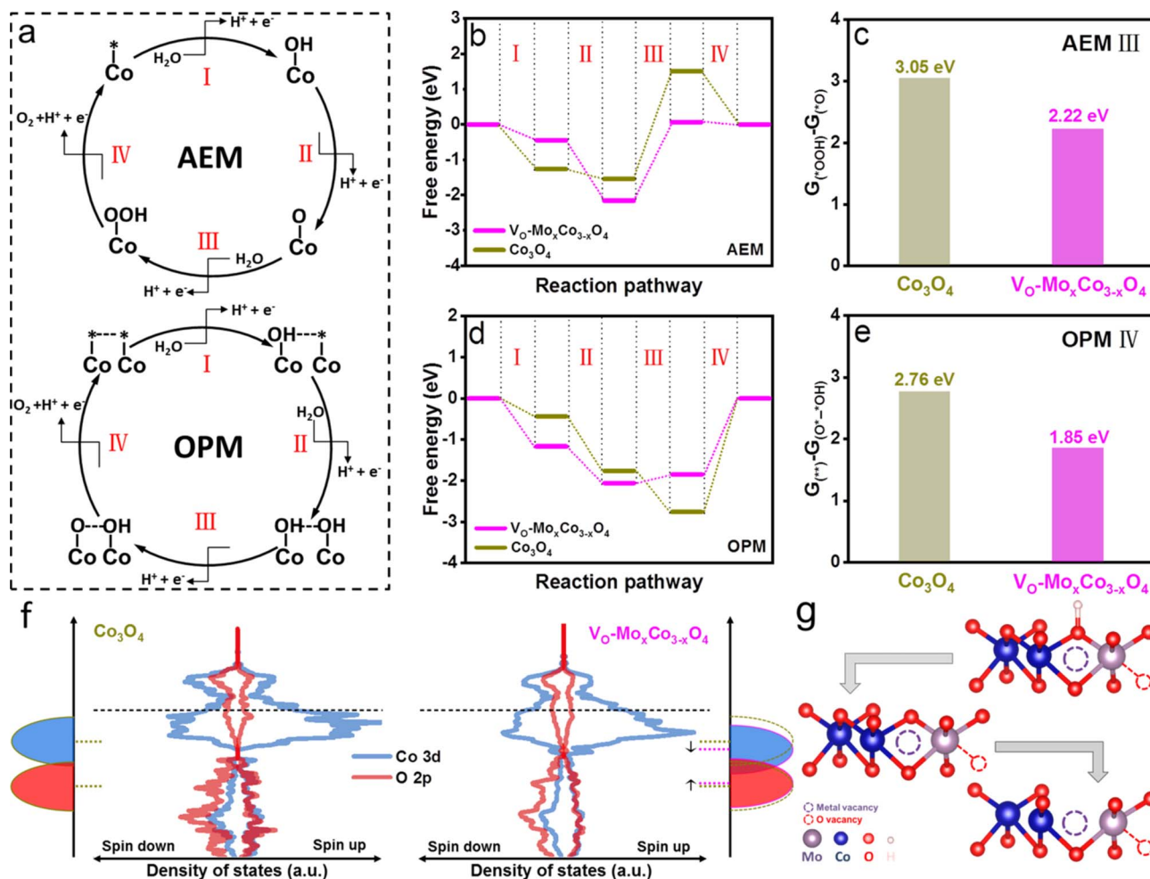
Fig. 4 (a) Schematic illustration of mechanisms for the OER through AEM and OPM pathways. (b) Gibbs free energy diagrams of the AEM pathway on V_{O-Mo_xCo_{3-x}O_4} and Co_3O_4 . (c) Histogram of free energy increases of Co_3O_4 and V_{O-Mo_xCo_{3-x}O_4} during the PDS of the AEM pathway (AEM III) at U = 1.23 V. (d) Gibbs free energy diagrams of the OPM pathway on V_{O-Mo_xCo_{3-x}O_4} and Co_3O_4 . (e) Histogram of free energy increases of Co_3O_4 and V_{O-Mo_xCo_{3-x}O_4} during the PDS of the OPM pathway (OPM IV) at U = 1.23 V. (f) The curves of density of states and schematic diagrams of Co 3d and O 2p orbitals in V_{O-Mo_xCo_{3-x}O_4} and Co_3O_4 . (g) The optimized structures of key intermediates adsorbed on the surface of V_{O-Mo_xCo_{3-x}O_4} during the OPM pathway.
