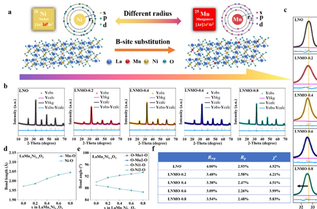
Fig. 3 (a) B-site substitution diagram of LNMO- x solid solution. (b) XRD patterns of LaMn_xNi_{1-x}O_3 ( x = 0, 0.2, 0.4, 0.6, 0.8 ) with their Rietveld refinement results. (c) Partial enlargement of the XRD pattern. (d) Change in bond length of LaMn_xNi_{1-x}O_3 ( x = 0, 0.2, 0.4, 0.6, 0.8 ). (e) Change in bond angle of LaMn_xNi_{1-x}O_3 ( x = 0, 0.2, 0.4, 0.6, 0.8 ). (f) Error analysis values of Rietveld data for the XRD pattern.
