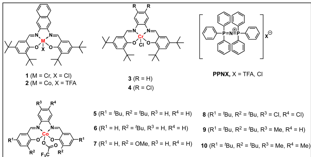
Fig. 1 Different M(Salophen)X ( M = \text{Co}, \text{Cr} ) metal complexes.
