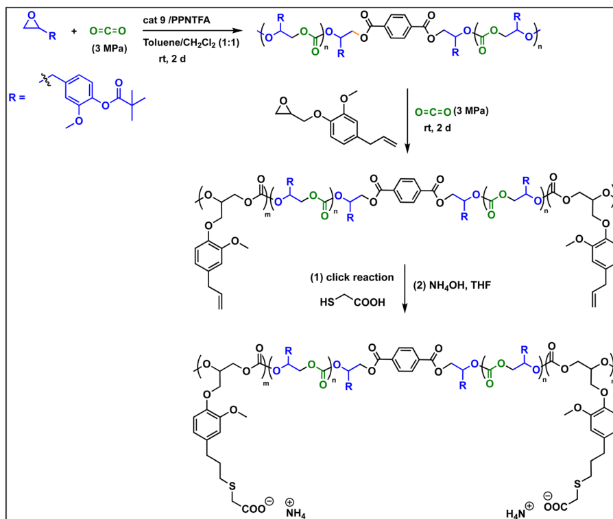
Scheme 5 Sequential block copolymer formation between (EuO/EGE)/CO 2 .
