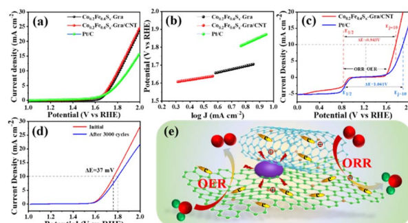
Fig. 4 (a) LSV curves of the catalysts for the OER in 0.1 M KOH with a scanning rate of 5 \text{ mV s}^{-1} and rotating rate of 1600 rpm. (b) Tafel plots of the catalysts for OER. (c) Overall LSV curves of the catalysts at the rotating rate of 1600 rpm. (d) LSV curves of the \text{Co}_{0.2}\text{Fe}_{0.6}\text{S}_x\text{-Gra/CNT} for the OER before and after 3000 cycles. (e) The interaction schematic illustration of the metal sulfides and heteroatoms-doped graphene and CNTs for the ORR and OER processes.
