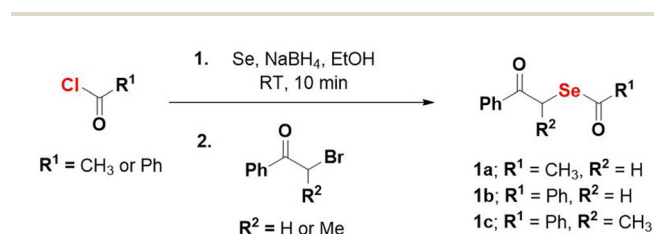
Scheme 1 Synthesis of selenium donors 1a , 1b and 1c . Overall yields were 28–58%.
