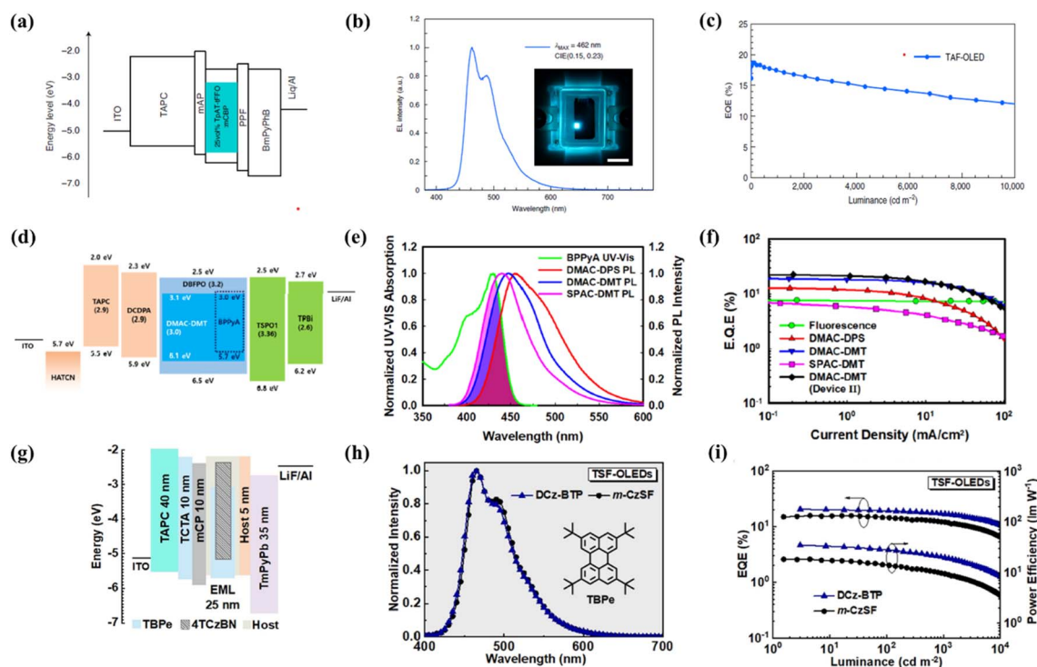
Fig. 4 Blue hyperfluorescent OLEDs. (a–c) Device structure, electro luminescence spectra and efficiency of the mCP:TpAT-tFFO:TBPe emissive system. Reproduced with permission from ref. 54, Nature , 2020. (d–f) Device structure using DPEPO:DMAC-DMT:BPPyA as an emissive layer, overlap of absorption of BPPyA with the emission spectra of the TADF sensitizers and EQE of all the devices. Reproduced with permission from ref. 56, American Chemical Society, 2018. (g–i) Device structure of the hyperfluorescent device with the 4TCzBN sensitizer and TBPe emitter, electro luminescence spectra and EQE–luminance–power efficiency plots. Reproduced with permission from ref. 58, John Wiley and Sons, 2022.
