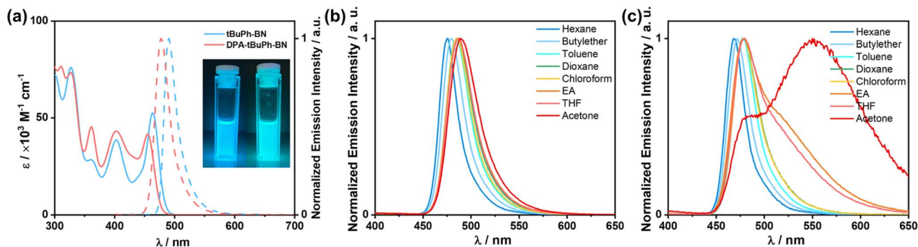
Fig. 4 (a) UV-vis absorption spectra and PL spectra of tBuPh-BN and DPA-tBuPh-BN in toluene at 300 K; inset: photos of tBuPh-BN (right) and DPA-tBuPh-BN (left) in toluene excited at 365 nm. PL spectra of (b) tBuPh-BN and (c) DPA-tBuPh-BN in different solvents at 300 K. ( \lambda_{\text{exc}} = 340 nm).
