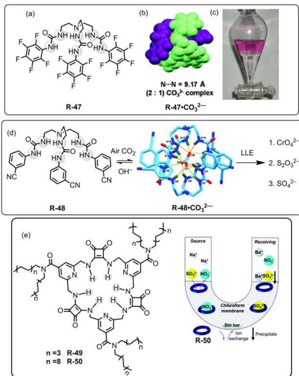
Fig. 16 (a) Chemical structure of the receptor R-47. (b) Representation of the assembly of R-47·CO 3 2- . (c) Visualization of SO 4 2- extraction using phenolphthalein through the R-47·CO 3 2- complex. (Reproduced from ref. 81. Copyright 2012, The Royal Society of Chemistry.) (d) Schematic representation of LLE by R-48 (Reproduced from ref. 82. Copyright 2014, Wiley.) (e) Chemical structures of the receptors R-49 and R-50. Illustration of the general setup for the U-tube experiments used to test the ability of R-50 to act as a carrier for SO 4 2- . (Reproduced from ref. 83. Copyright 2020, The Royal Society of Chemistry.)
