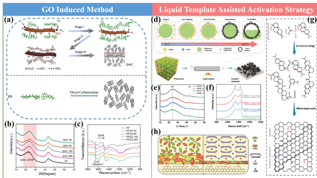
Fig. 7 (a) Proposed formation mechanism of GHGs under different conditions, (b and c) XRD patterns and FTIR spectra of GHGs, (d) diagram for the preparation of "egg puff"-like HC, (e and f) XRD patterns and Raman spectra of SNQLs, (g) diagram of the structure transformation and (h) diagram of SEI in different electrolytes.
