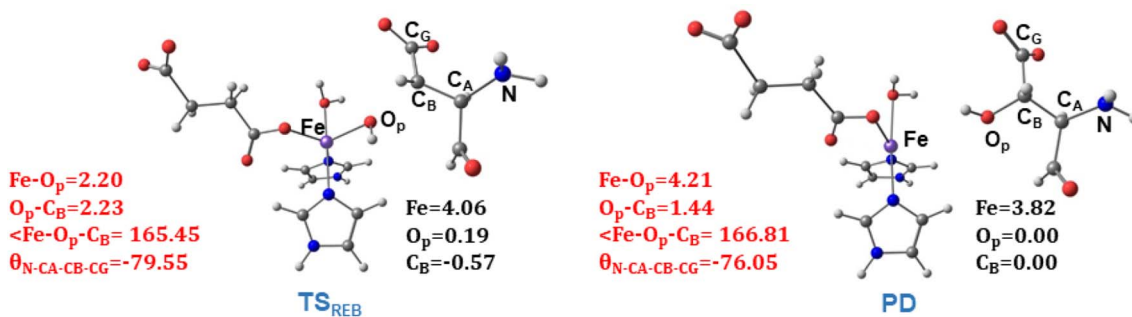
Fig. 10 Geometric parameters (red) and spin densities (black) of optimized stationary points in rebound hydroxylation step.
