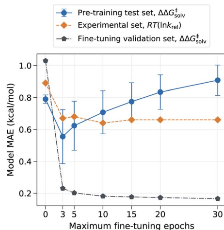
Fig. 4 Model MAE vs. the number of fine-tuning epochs. The model is trained with no additional feature. The error on the pre-training set is evaluated on the reaction split test set, and the error on the fine-tuning set is evaluated on the random split validation set.
