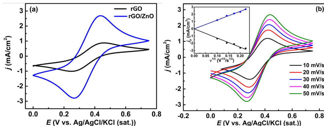
Fig. 3 (a) CVs obtained at the rGO and rGO/ZnO-modified GCE at a \nu of 50 mV s ^{-1} and (b) CVs obtained at rGO/Ag at different \nu values (inset: plot of the variation in anodic and cathodic j_p as a function of \nu^{1/2} ) in a 5 mM [Fe(CN) _6 ] ^{3-} /[Fe(CN) _6 ] ^{4-} solution containing 0.1 M KCl.
