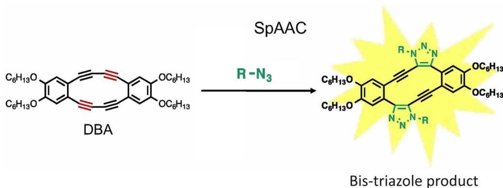
Fig. 25 Bis-triazole product is formed when octadecyldibenzotriazolo [12] annulenes undergo strain-promoted-azide-alkyne cycloaddition. Reproduced from ref. 159 with permission from John Wiley and Sons, copyright 2019.
