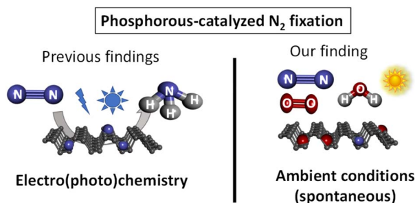
Scheme 1 Previous work on phosphorous-catalyzed \text{N}_2 fixation and the spontaneous fixation on elemental phosphorous under ambient conditions reported herein. Ammonia is obtained after hydrolysis.
