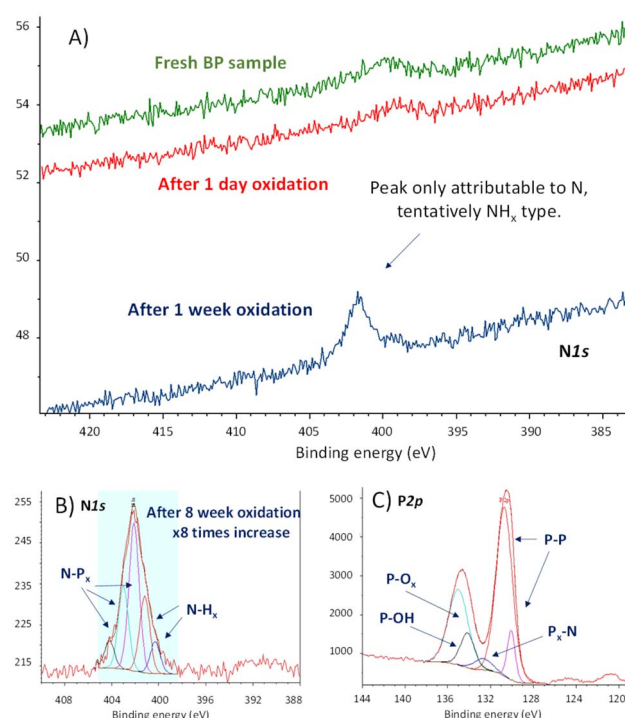
Fig. 2 (A) \text{N}1\text{s} X-ray photoelectron spectra (XPS) of fresh FL-BP (green line), and left under ambient conditions for 1 day (red line) and 1 week (blue line) respectively, managed and recorded at HIERN laboratory. (B) Deconvoluted high-resolution \text{N}1\text{s} XPS of FL-BP left under ambient conditions for 8 weeks, managed and recorded at ITQ-UPV/CSIC laboratory. (C) Deconvoluted high-resolution \text{P}2\text{p} XPS of the previous sample (B).
