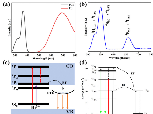
Fig. 3 PL properties of 2%Bis@20%Yb, 7%Er. (a) PL ( \lambda_{\text{ex}} = 370 nm) and PLE ( \lambda_{\text{em}} = 690 nm) spectra; (b) PL ( \lambda_{\text{ex}} = 980 nm) spectrum; (c) schematic diagram of the energy-transfer mechanism of \text{Bi}^{3+} in core-shell NCs; (d) schematic diagram of the energy-transfer mechanism of \text{Yb}^{3+} – \text{Er}^{3+} in core-shell NCs.
