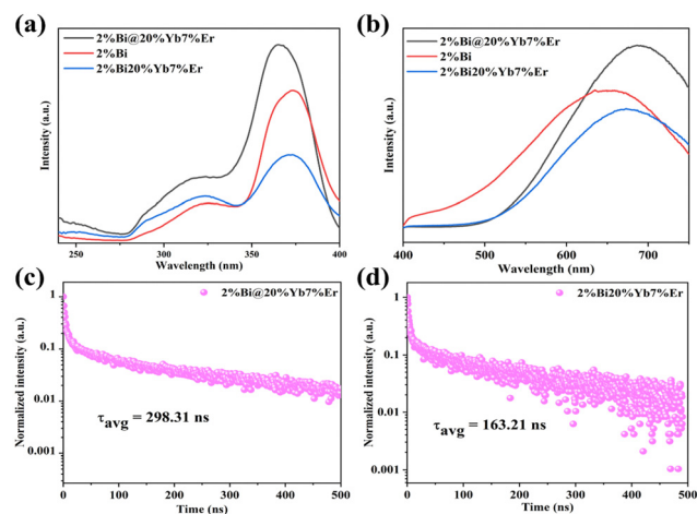
Fig. 4 (a) and (b) The PLE and PL spectra of 2%Bis@20%Yb, 7%Er, 2%Bis and 2%Bis, 20%Yb, 7%Er NCs; (c) and (d) PL decay curves of 2%Bis@20%Yb, 7%Er and 2%Bis, 20%Yb, 7%Er NCs emission at around 690 nm under 375 nm excitation.
