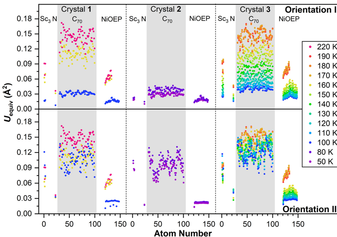
Fig. 4 The equivalent atom displacement parameters (ADPs, U_{\text{equiv}} ) of \text{Sc}_3\text{N}@C_{70} and NiOEP and their variation with temperature for orientation I (top panel) and orientation II (bottom panel). To guide the eye, the range of atom numbers corresponding to the carbon cage is shaded.
